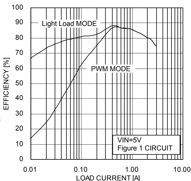
Figure 2. Efficiency (BD90535EFJ-C)
