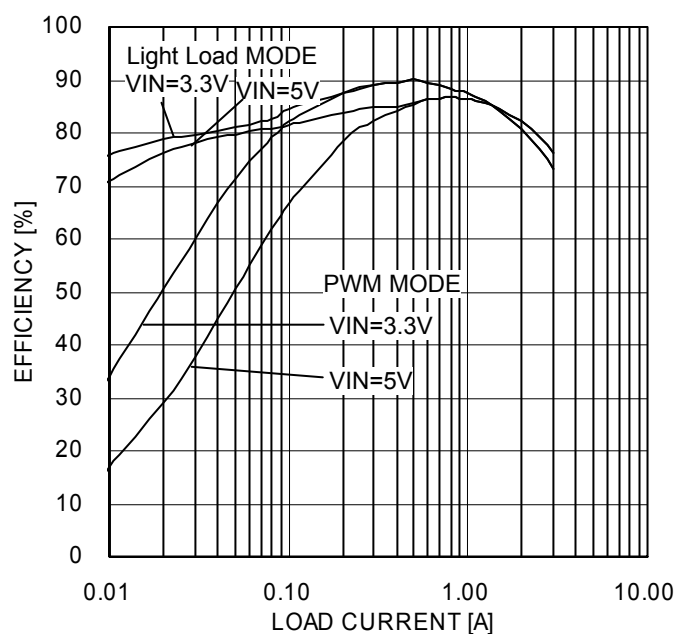
Figure 9. Efficiency(BD90538EFJ-C)
