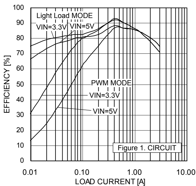
Figure 8. Efficiency(BD90535EFJ-C)
