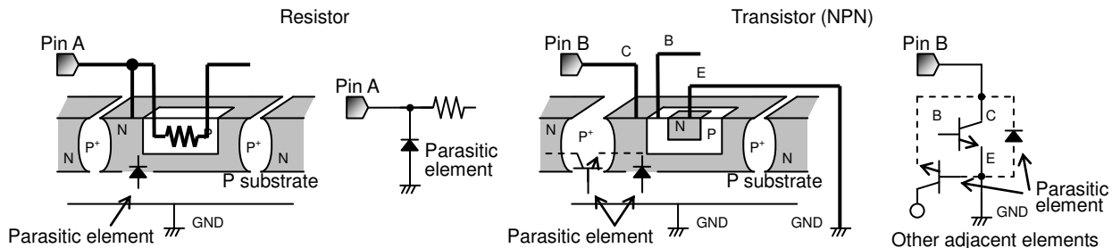
Fig.34 Simplified structure of monorisc IC
