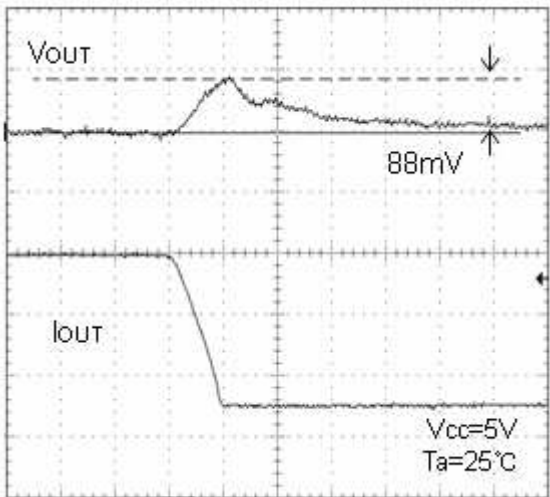
Fig.17 Transient response I_o=600\rightarrow100mA(10\mu s)
