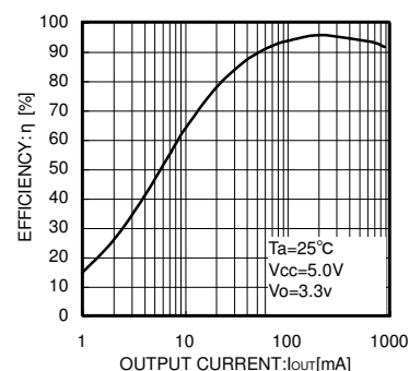
Fig.23 Efficiency
