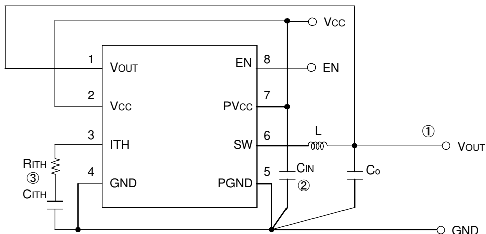
Fig.32 Layout diagram
