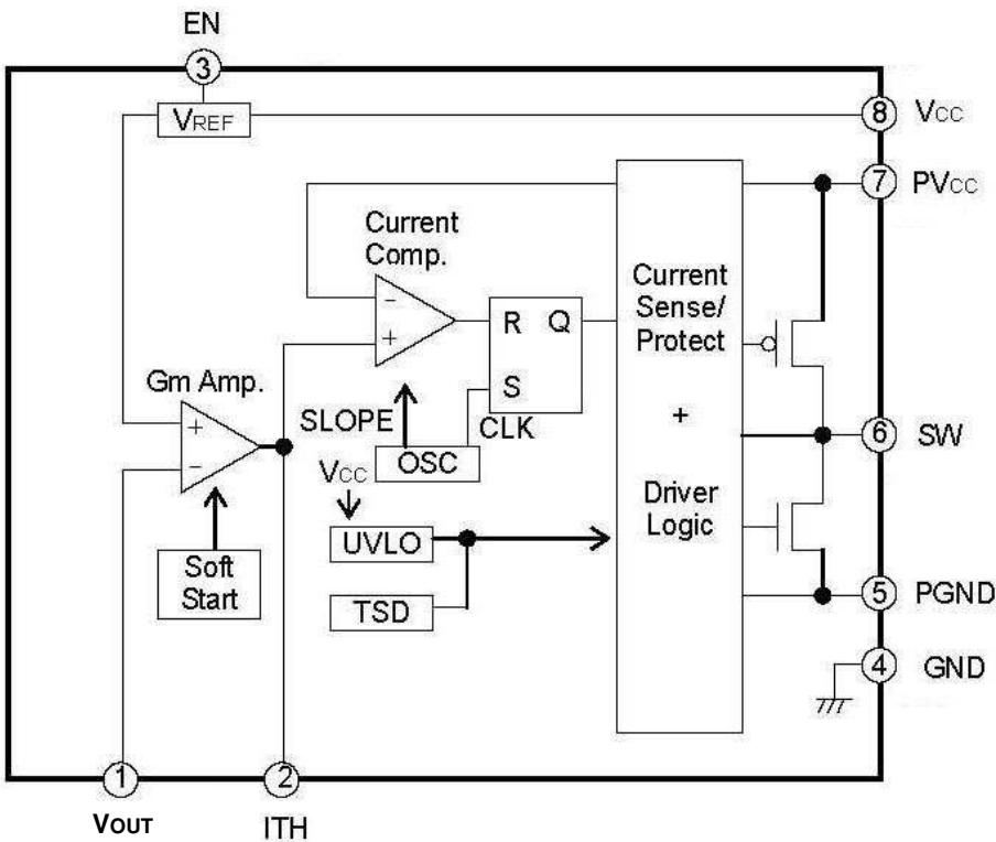
Fig.3 Block Diagram
