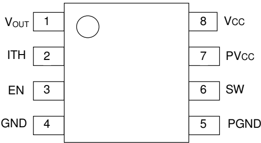
Fig.2 Pin Configuration
