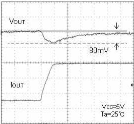
Fig.16 Transient response I_o=100\rightarrow600mA(10\mu s)
