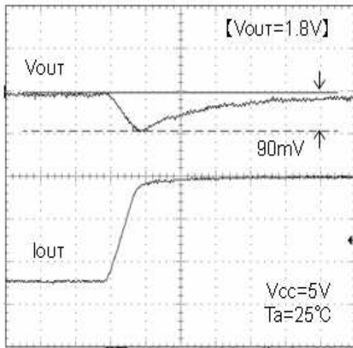
Fig.16 Transient response Io=100→600mA(10μs)
