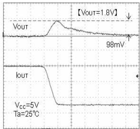
Fig.17 Transient response Io=600→100mA(10μs)
