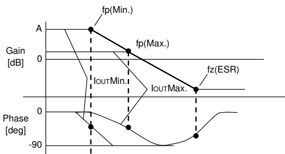
Fig.29 Open loop gain characteristics
