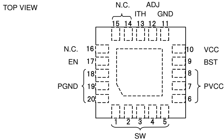
Fig.2 Pin configuration
