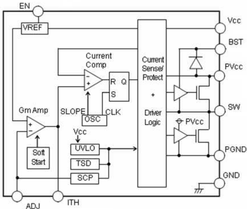
Fig.3 Block Diagram
