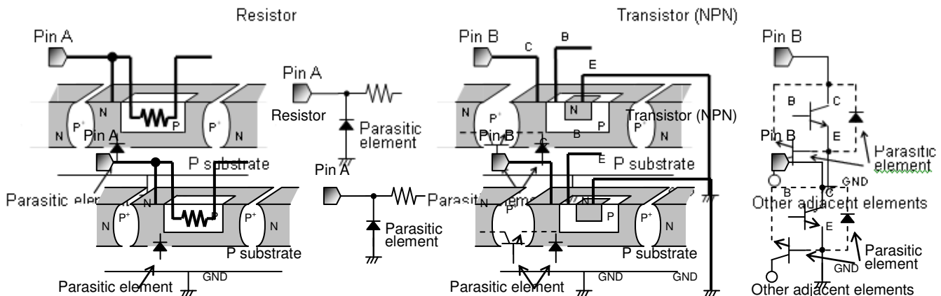
Fig.36 Simplified structure of monolithic IC
