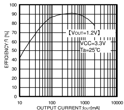
Fig.23 Efficiency
