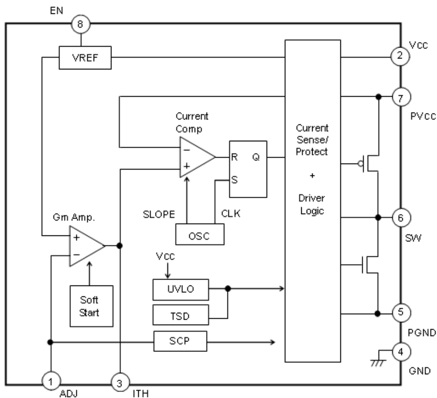
Fig.3 Block Diagram
