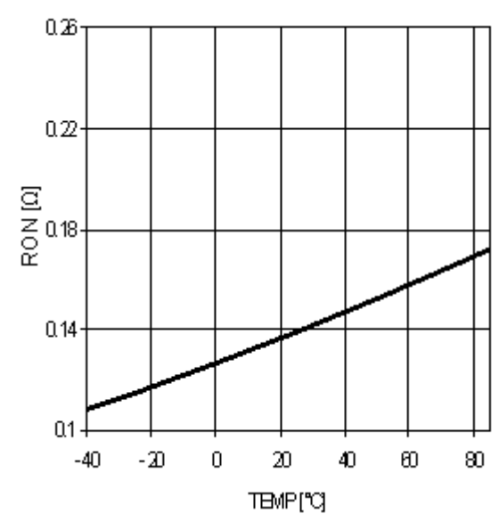
Fig.8 Hi,Low-Side On-resistance
