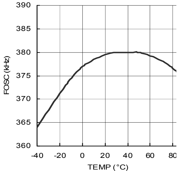
Fig.9 Operating Frequency
