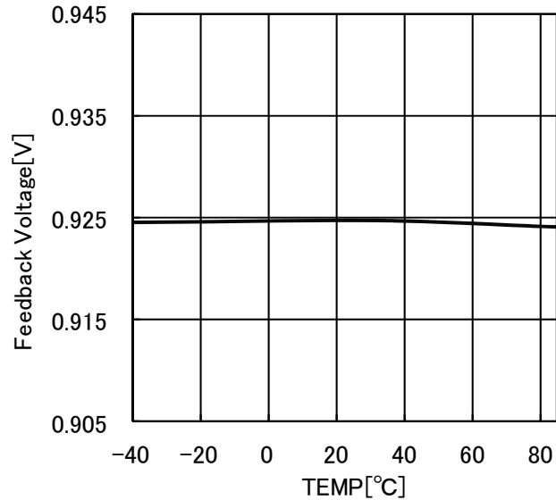
Fig.7 Feedback voltage
