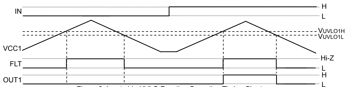
Figure 8. Input-side UVLO Function Operation Timing Chart
