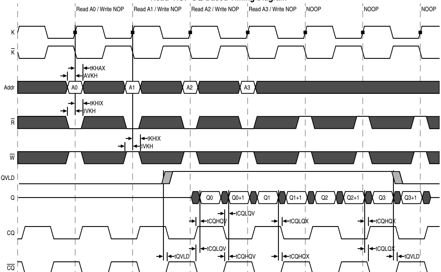
Read NOP CQ-Based Timing Diagram
