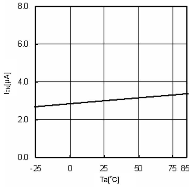
Fig.14 T_a - I_{EN}
