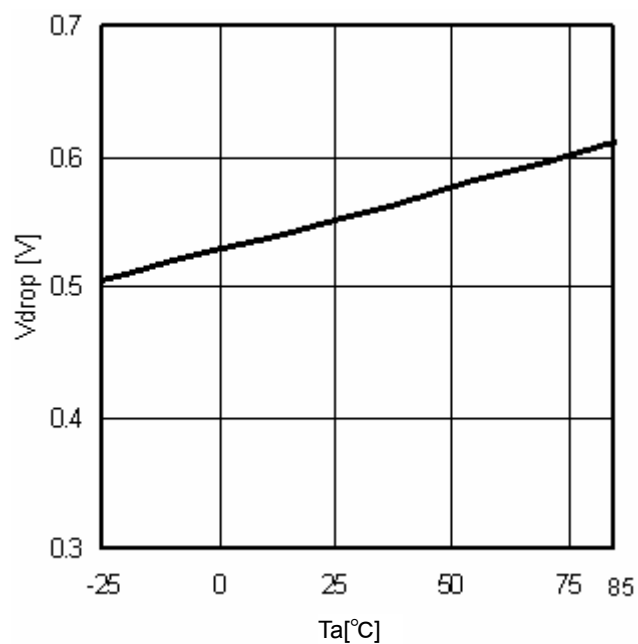
Fig.18 Minimum dropout Voltage1 ( V_{CC}=5\text{V} , I_O=-1.5\text{A} )
