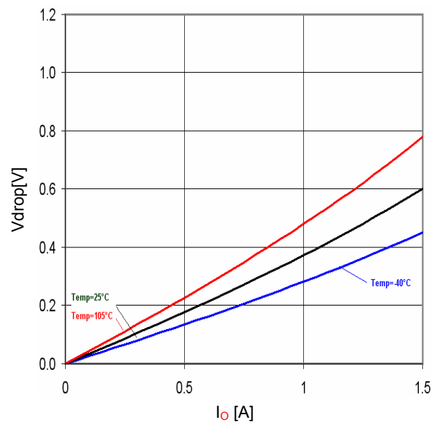
Fig.34 Minimum dropout Voltage 2 ( V_{CC}=4.5V , T_a=25^{\circ}C )
