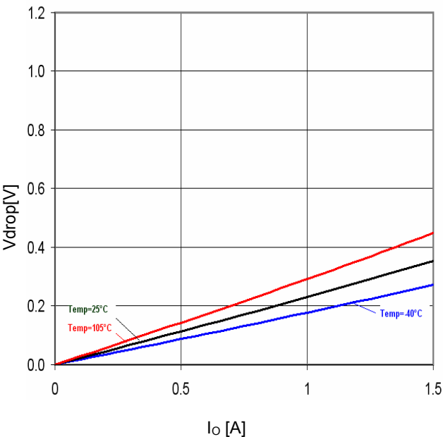
Fig.37 Minimum dropout Voltage 2 (V CC =10, Ta=25°C)
