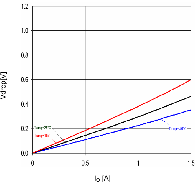
Fig.35 Minimum dropout Voltage 2 (V CC =6, Ta=25°C)
