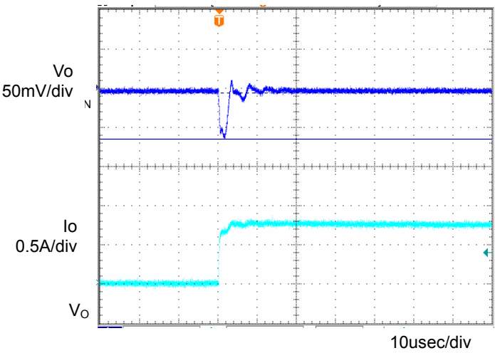
Fig.5 Transient Response (0→1.0A) Co=1 \mu F, Ta=-40°C
