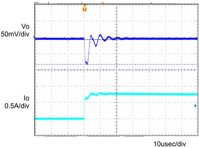
Fig.5 Transient Response (0→1.0A) Co=1 \mu F, Ta=105°C
