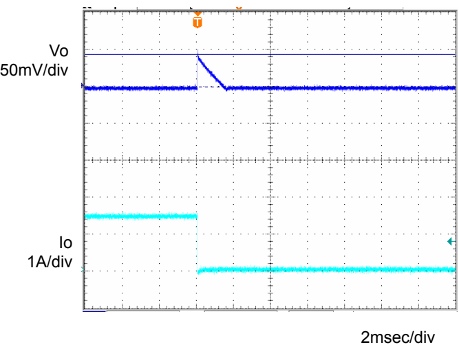
Fig.6 Transient Response (1.0→0A) Co=1 \mu F, Ta=-40°C
