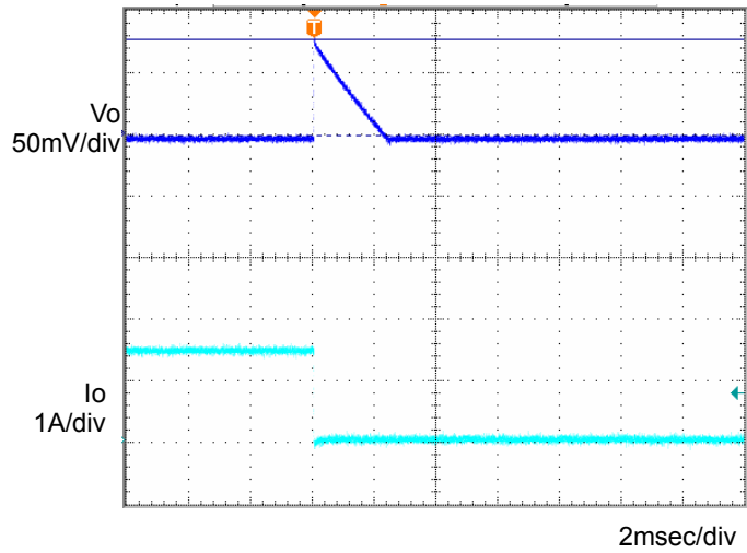
Fig.8 Transient Response (1.0→0A) Co=1μF,Ta=105°C
