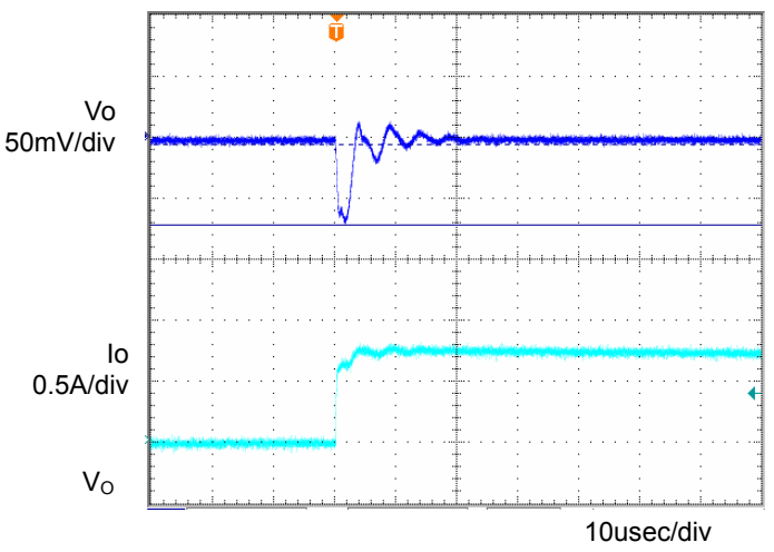
Fig.6 Transient Response (1.0→0A) Co=1 \mu F, Ta=25°C
