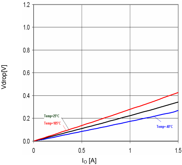
Fig.38 Minimum dropout Voltage 2 (V CC =12V, Ta=25°C)
