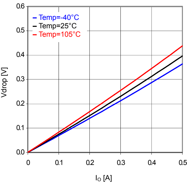
Fig. 34 Minimum dropout Voltage 1 ( V_{CC}=4.5\text{V} )
