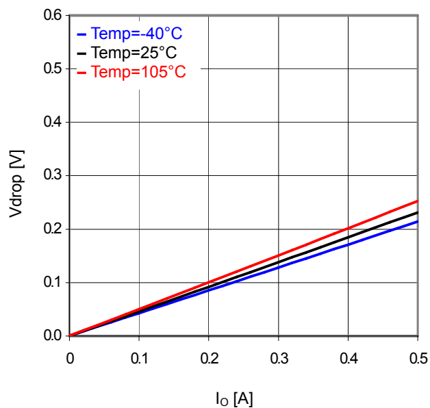
Fig. 38 Minimum dropout Voltage 5 (V CC =12.0V)
