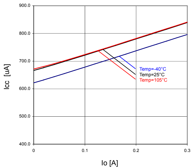
Figure 30. I_o - I_{CC}
