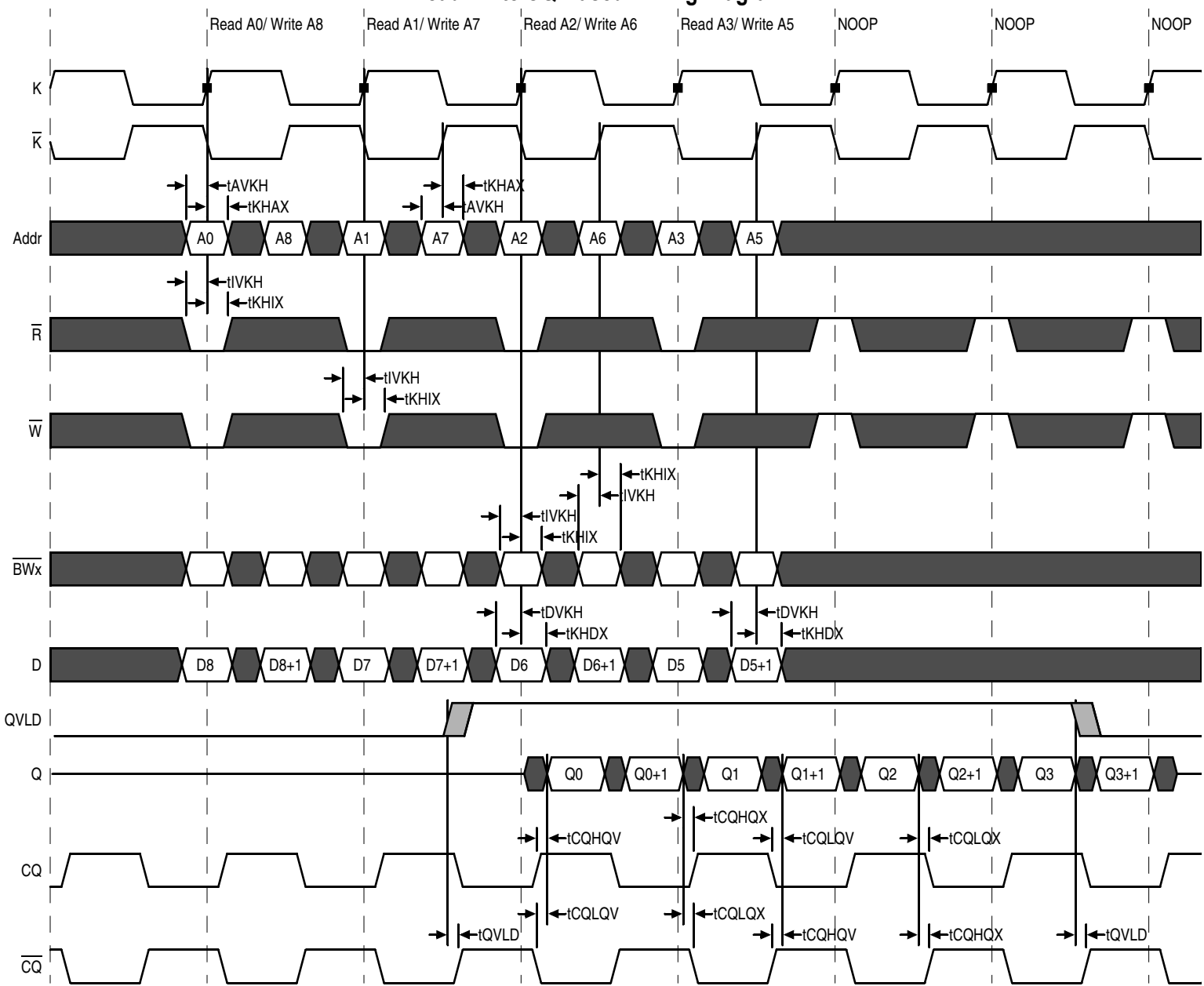
Read-Write CQ-Based Timing Diagram
