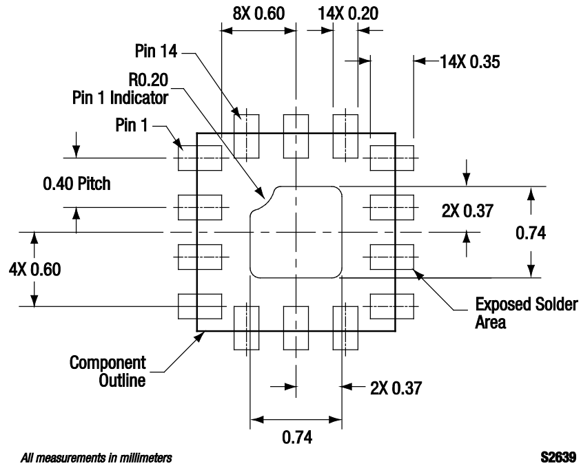
Figure 9. SKY13421-486LF PCB Layout Footprint (Top View)
