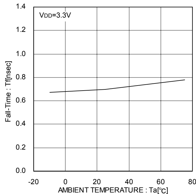
Figure 24. CLKOUT Fall-Time
