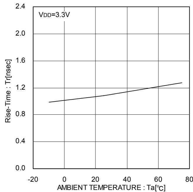
Figure 22. CLKOUT Rise-Time
