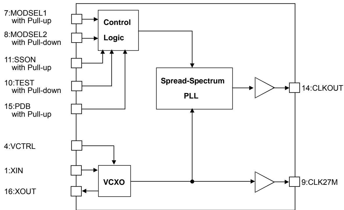
Figure 2. Block Diagram
