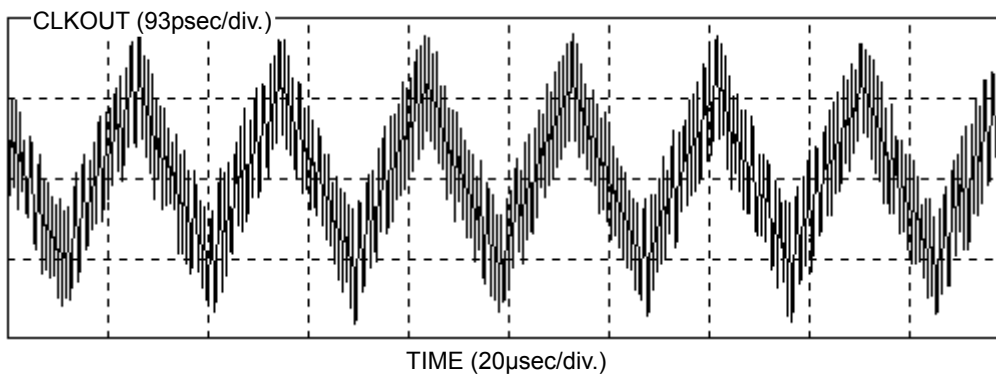
Figure 31. CLKOUT \pm 0.75\% Modulation Waveform
