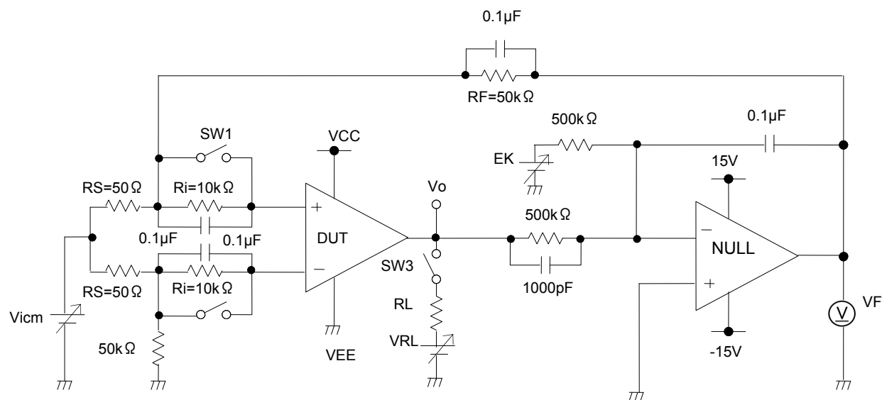
Figure 21. Test circuit 1
