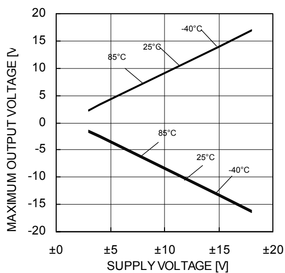
Figure 5. Maximum Output Voltage – Supply Voltage (RL=2kΩ)
