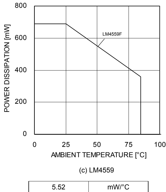
Figure 28. Thermal resistance and Derating Curve
