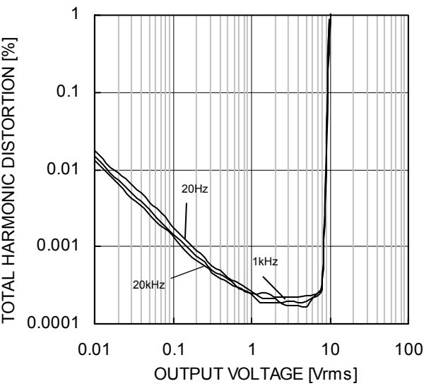
Figure 18. Total Harmonic Distortion - Output Voltage (VCC/VEE=±15V, RL=2kΩ)
