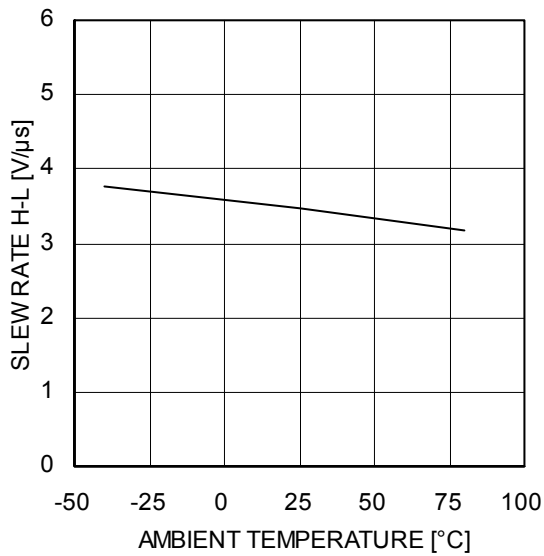
Figure 14. Slew Rate H-L – Ambient Temperature (VCC/VEE=±15V, RL=2kΩ, CL=100pF)
