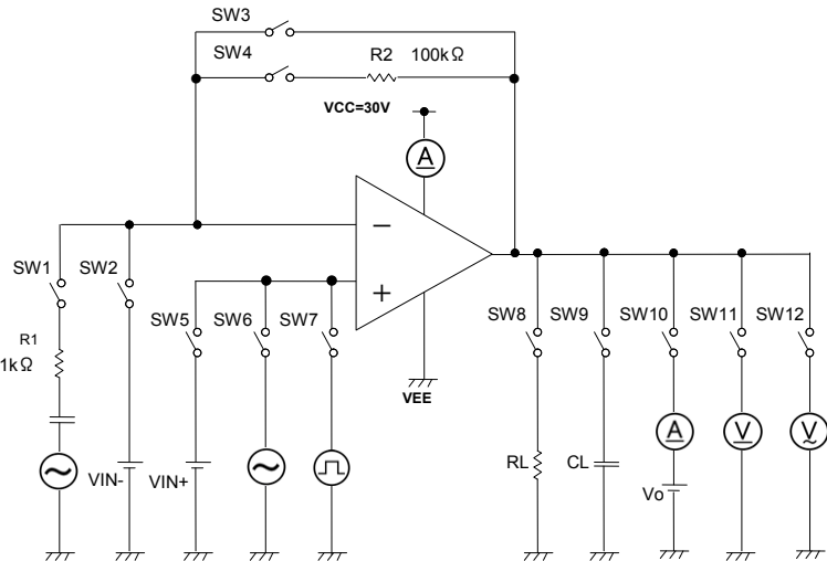
Figure 22. Test circuit2
