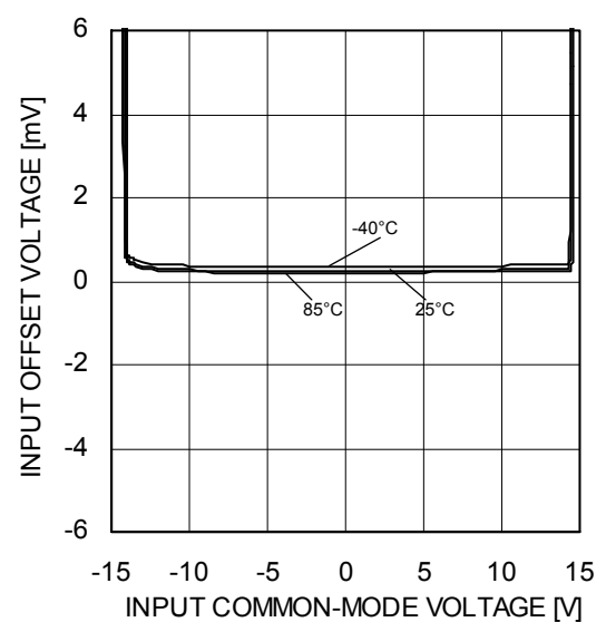
Figure 9. Input Offset Voltage – Input Common-mode Voltage (VCC/VEE=±15V)
