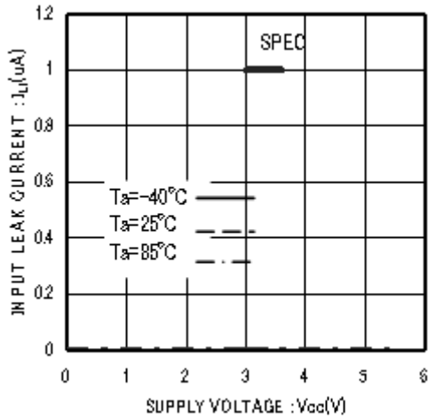
Figure 6. Input leak current I_{LI} (CS,SK,DI)
