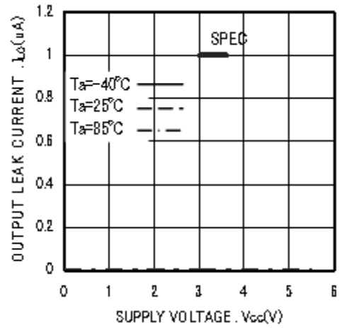
Figure 7. Output leak current I_{LO} (DO)
