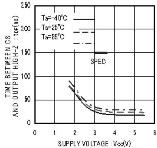
Figure 21. Time from CS to High-Z tOZ
