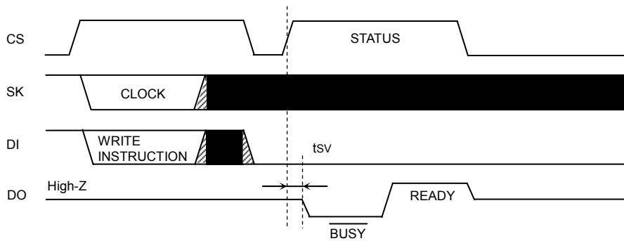
Figure 39. \overline{\text{R}} / \overline{\text{B}} status output timing chart
