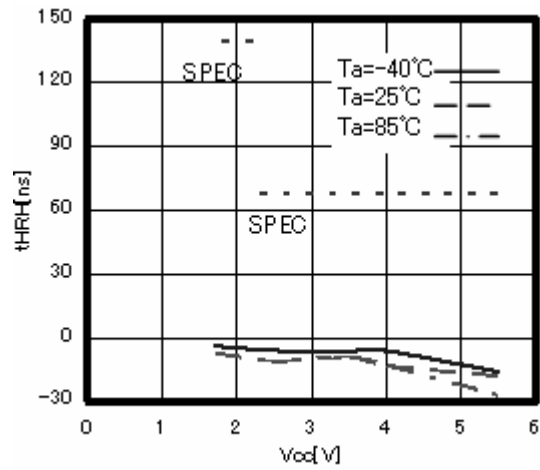
Figure 27. \overline{\text{HOLD}} release hold time tHRH
