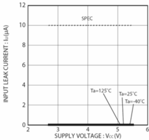
Figure 7. Input leak current I_{IL} (CS, SK, DI)
