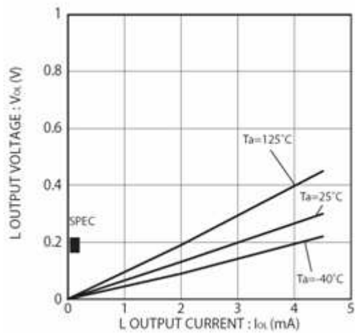
Figure 3. L output voltage V_{OL} - I_{OL} ( V_{CC}=2.7\text{V} )
