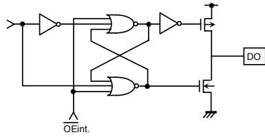
Figure 34. Output circuit (DO)
