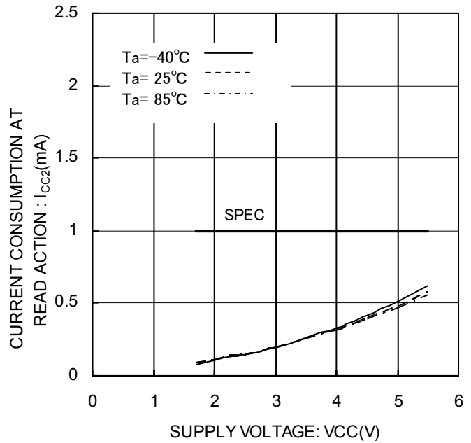
Figure 17. Current consumption at READ action I_{CC2}(READ, f_{SK}=3MHz)
