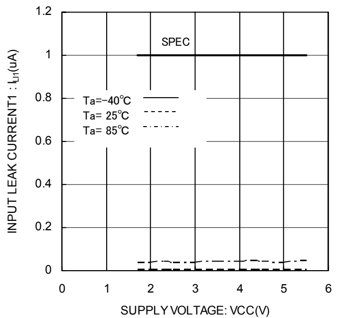
Figure 11. Input leak current1 I_{LI1} (SK)
