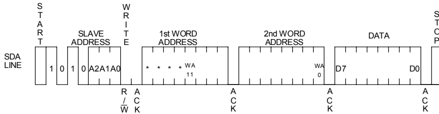
Figure 35. Byte write cycle
