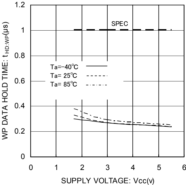
Figure 31. WP Hold Time t_{HD:WP}
