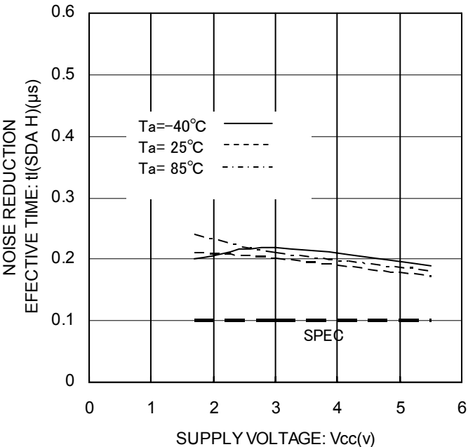
Figure 29. Noise Spike Width t_I (SDA H)
