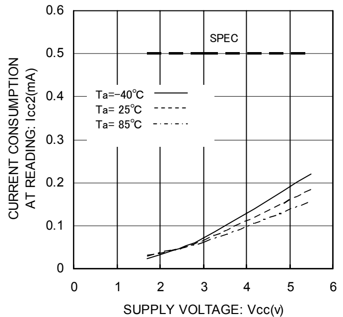
Figure 11. Operating Current at READ operation ICC2 ( f_{SCL}=400kHz )
