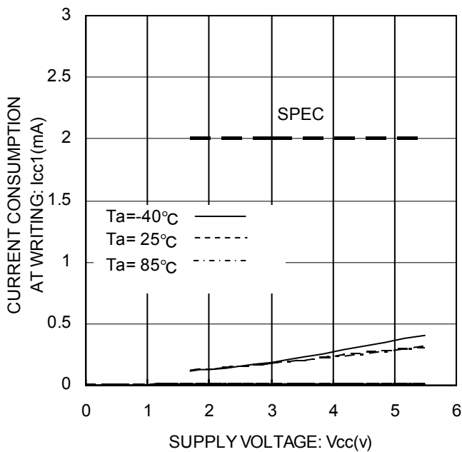
Figure 10. Operating Current at WRITE operation ICC1
