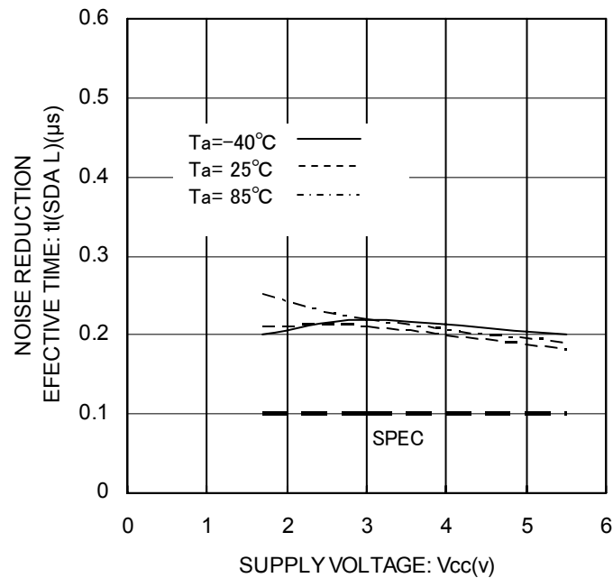
Figure 30. Noise Spike Width t_I (SDA L)
