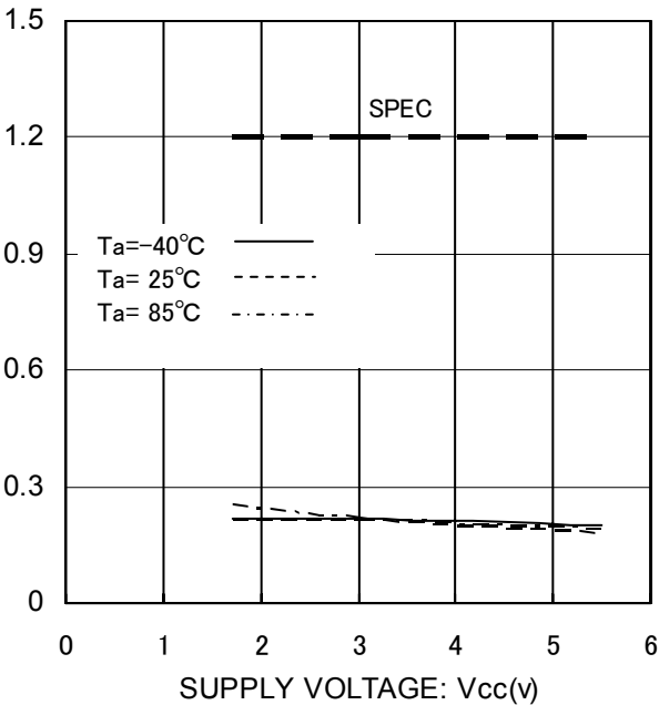
Figure 15. Data Clock Low Period t_{LOW}
