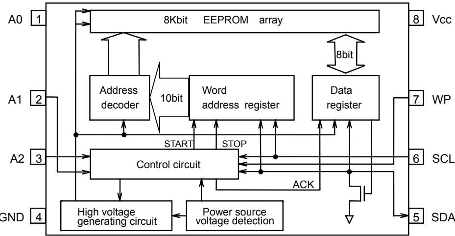
Figure 3. Block diagram
