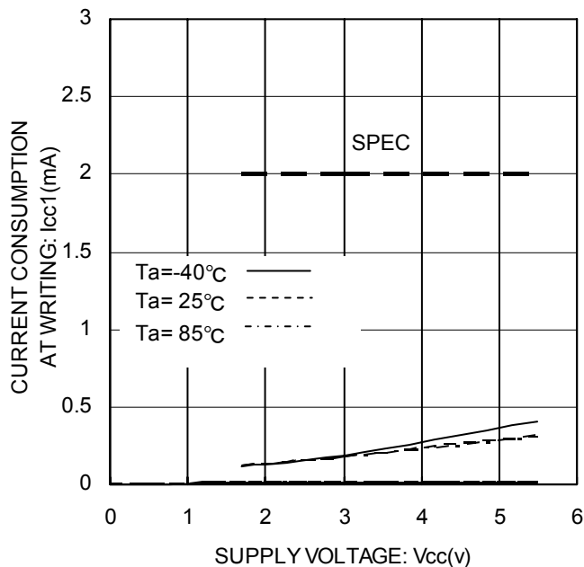
Figure 10. Operating Current at WRITE operation ICC1 ( f_{scl}=400kHz )
