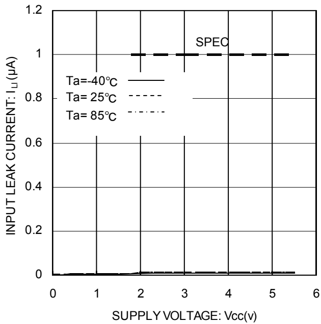
Figure 8. Input Leakage Current I_{II} (A2, SCL, WP)
