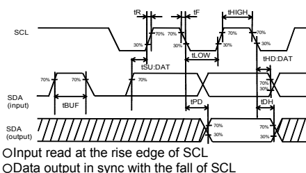
Figure 2-(a). Sync data input / output timing
