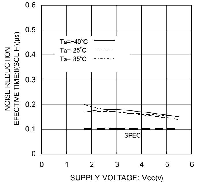
Fig 27. Noise Spike Width t_I(\text{SCL H})
