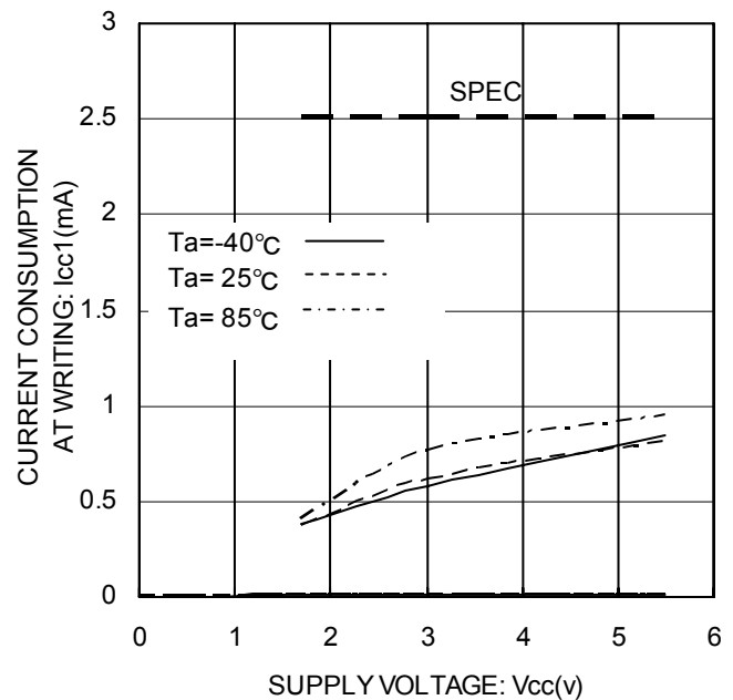
Figure 11. Operating Current at READ operation ICC2 ( f_{scl}=400kHz )
