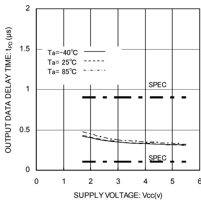
Figure 23. 'H' Output Data Delay Time t_{PD1}
