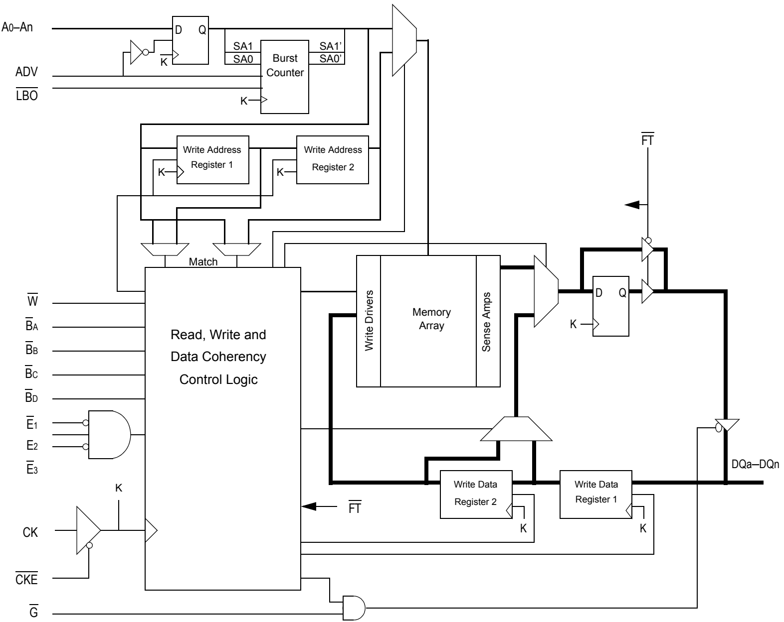
GS8160Z18/36B NBT SDRAM Functional Block Diagram
