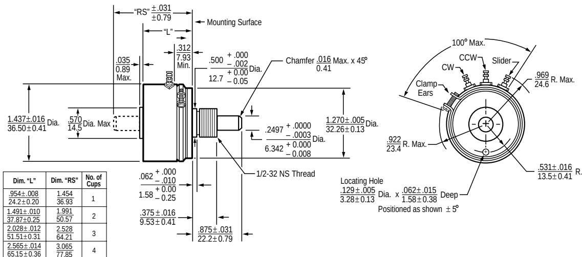
Model 5401 - Bushing Mount
