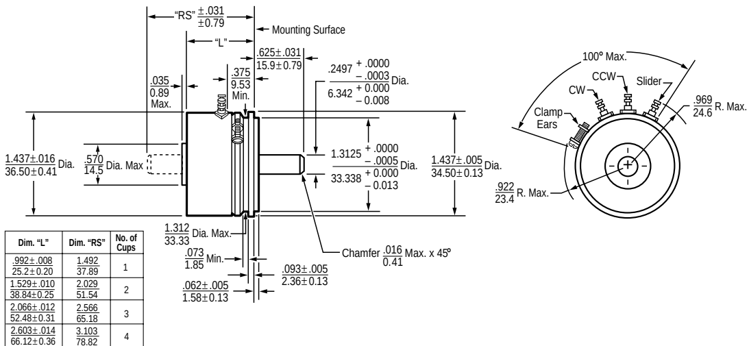
Model 5403 - Servo Mount
