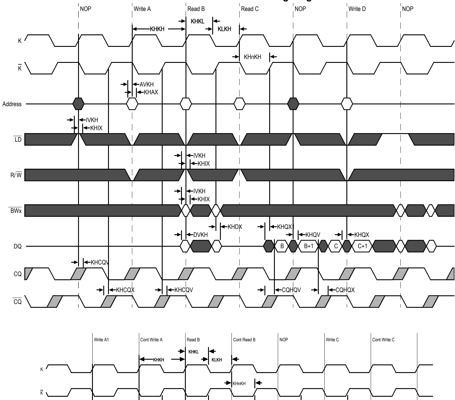
K and \bar{K} Controlled Write First Timing Diagram
