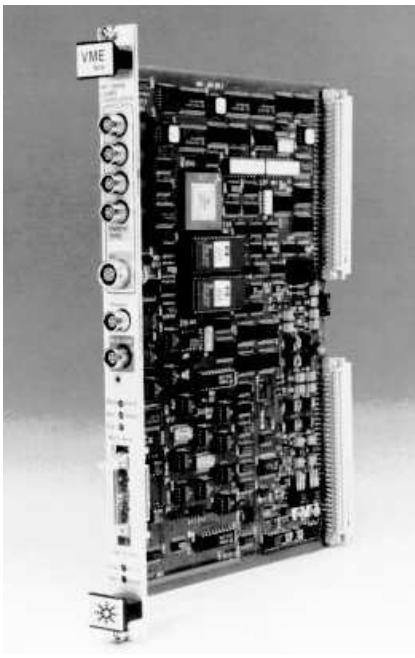
Improve system accuracy and repeatability using Agilent 10896B VMEbus laser compensation electronics.
