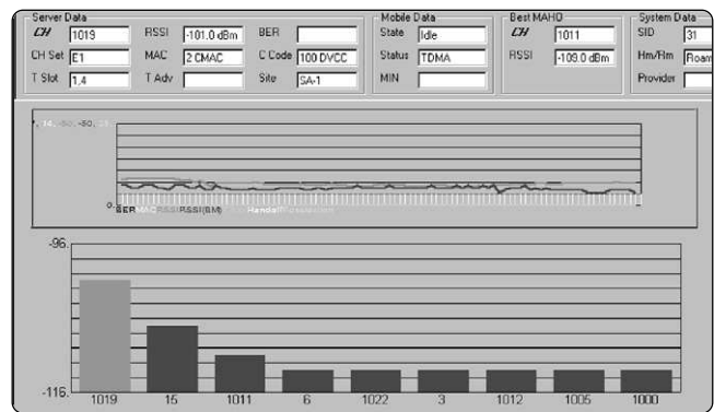
Figure 2. Phone measurements
