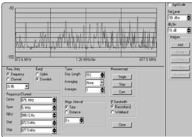
Figure 6. Spectrum
