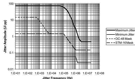
Figure 15. E4422B/N1015A Capability (2.4–3.2 Gb/s)
