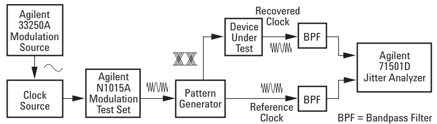
Figure 2. Block diagram for jitter transfer measurements
