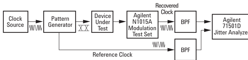
Figure 11. Measurement configuration for jitter generation
