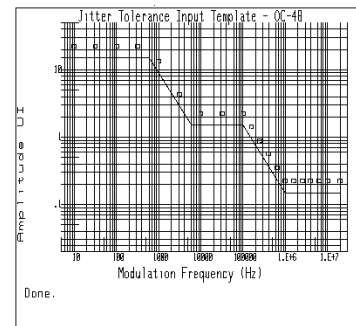
Figure 9. Jitter tolerance test with a 50% margin
