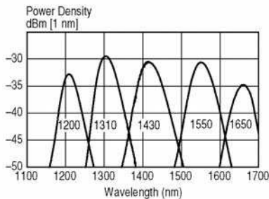
Characteristic spectra in single EELED configurations
