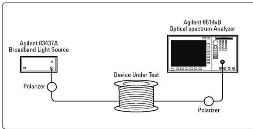
Test setup of a PMD measurement using the wavelength-scanning method.
