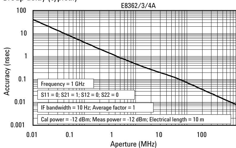
Group delay (typical)
