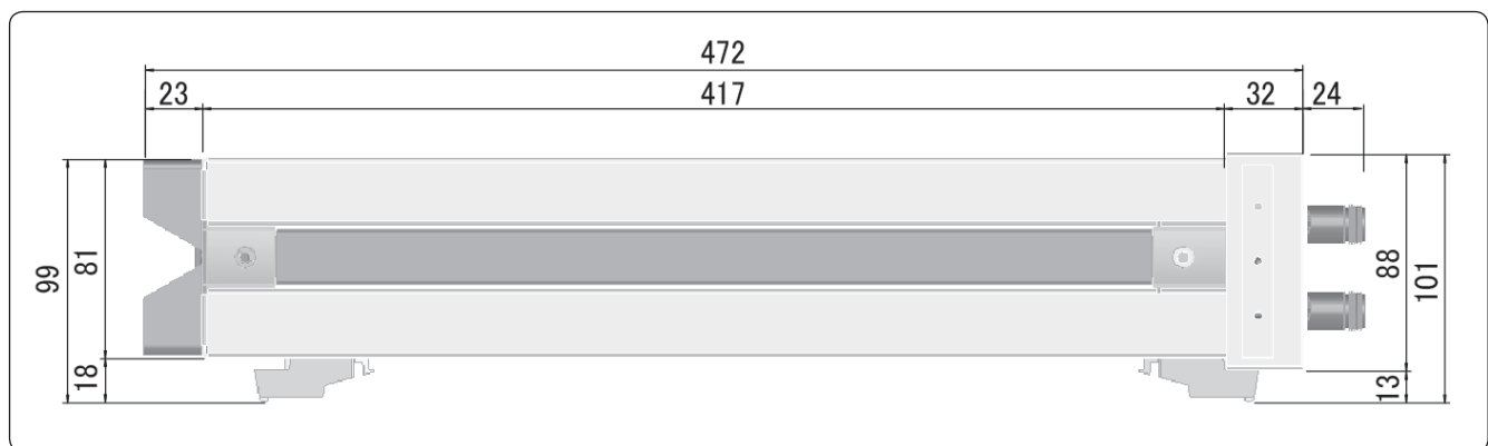
Figure 2-4. Dimensions (side view, with Option E5091A-009, in millimeters, nominal)
