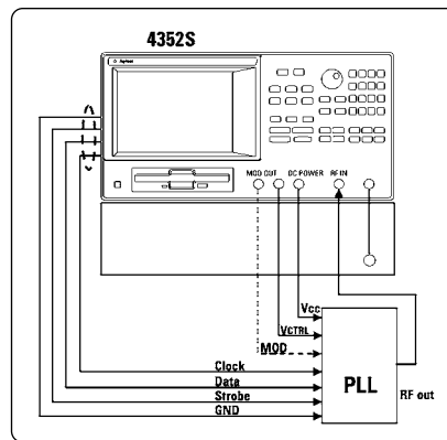
PLL measurement example
