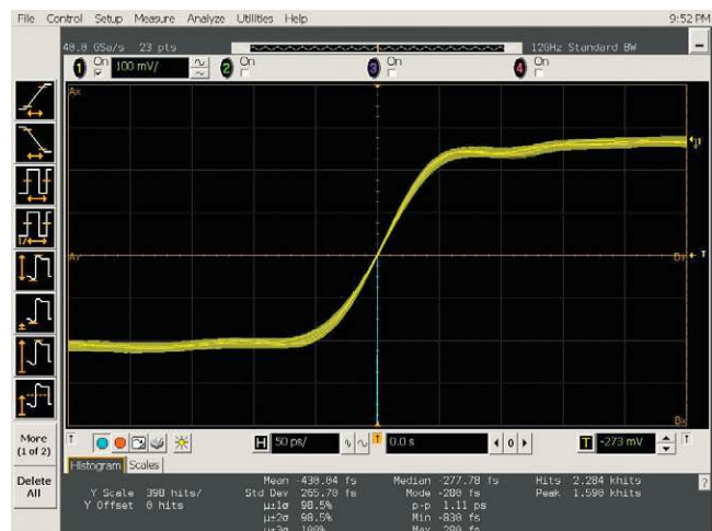
Figure 8. With the industry's lowest trigger jitter – less than 500 \text{ fs rms} (typically, less than 200 \text{ fs rms} on 5 \text{ Gb/s} PRBS signal) – the DSA80000B facilitates accurate waveform viewing of multiple waveforms.
