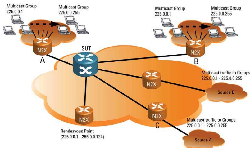
Figure 1: Scalability Test Scenario for PIM
