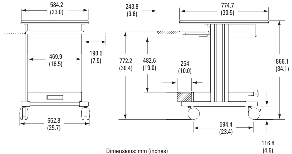
Figure 20. Agilent 1184A testmobile cart dimensions.
