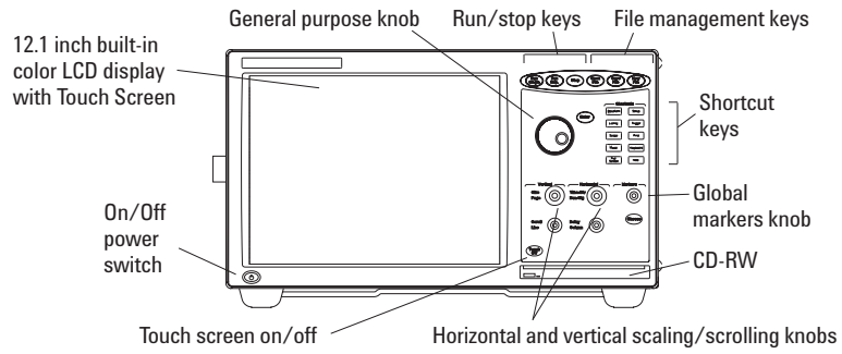
Figure 15. Agilent 16902A front panel
