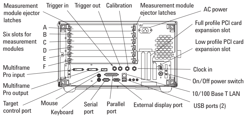
Figure 16. Agilent 16902A back panel
