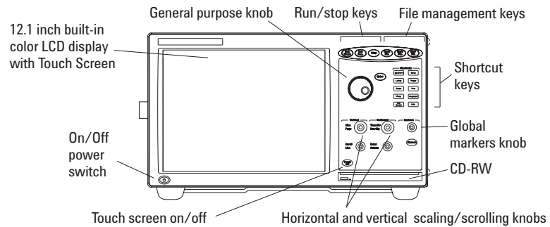
Figure 17. Agilent 16903A front panel
