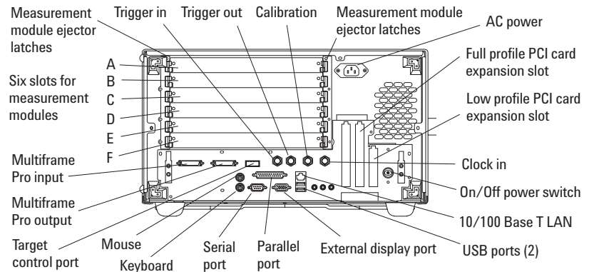
Figure 14. Agilent 16900A back panel
