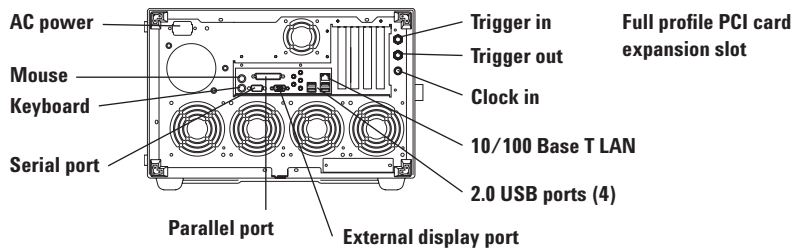
Figure 10. 16901A back panel
