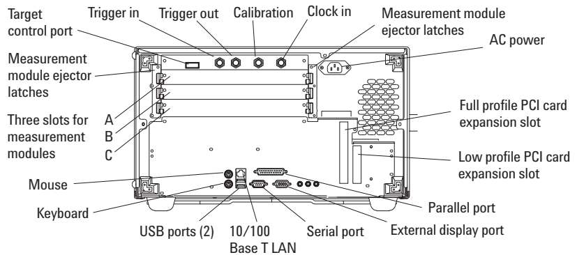
Figure 18. Agilent 16903A back panel
