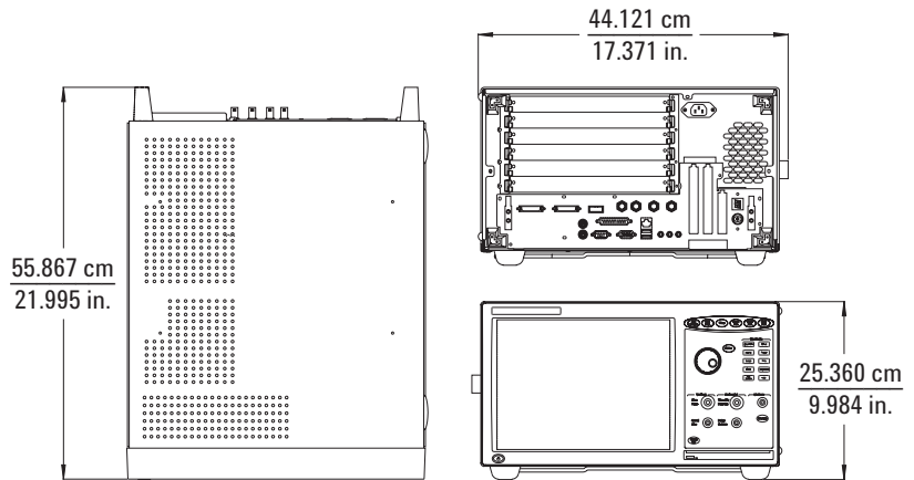
Figure 12. 16900A/16902A/16903A exterior dimensions
