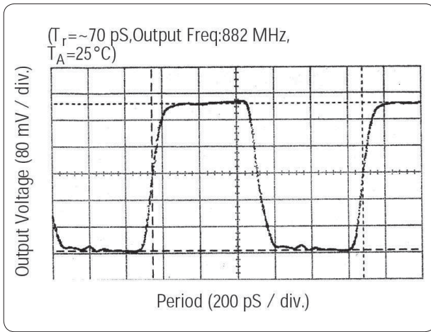
Figure 6. Typical output voltage waveform
