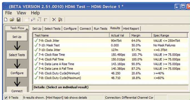
Figure 6. The HDMI electrical test software results report documents your test, indicates the pass/fail status, the test specification range, the measured values, and the margin.
