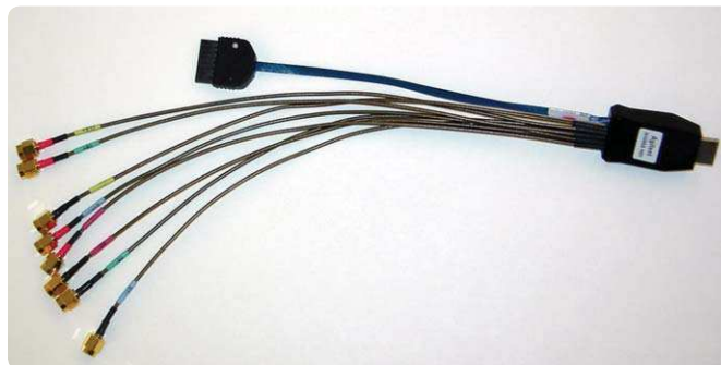
Figure 5a. The Agilent N1080A H01 HDMI test fixture.
