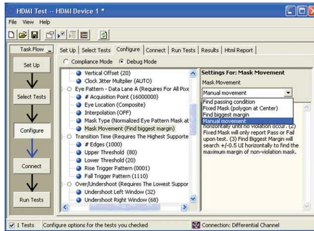
Figure 3. In configuring the tests, you define the device to test, its configuration, and how the oscilloscope is connected. Shown here is the N5399A's Debug Mode selection for Eye analysis.
