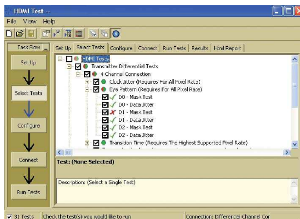
Figure 2. The Agilent automated test engine guides you quickly through selecting and configuring tests, setting up the connection, running the tests, and viewing the results. You can easily select individual tests or groups of tests with a mouse-click. Also easily seen is the test status for the device under test.
