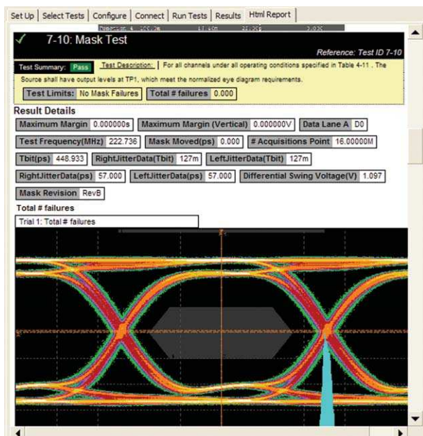
Figure 8. Summary Report Detail: the N5399A software's summary report yields all the screen shots of all the measurements that have been performed. In this figure you can see the Data-Eye. Observe the clear status and description at top and the measurement data just above the eye.
