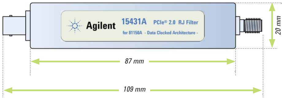
Figure 2. 15431A dimensions
