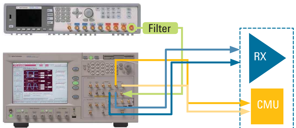
Figure 1. Test setup of a J-BERT with the 81150A for LF noise; the filtered signal from the 81150A is used as delay control input for the J-BERT. ISI and channel effects are merged into the signal path of the J-BERT by using the built-in trace 2.
