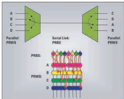
Figure 3. MUX/DEMUX application: relationship between PRBS and PRWS
