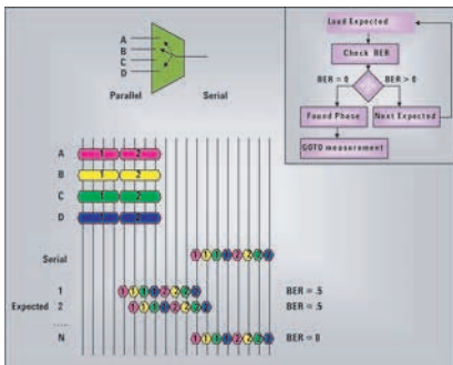
Figure 4. Mechanism of auto-phase and auto-delay assignment
