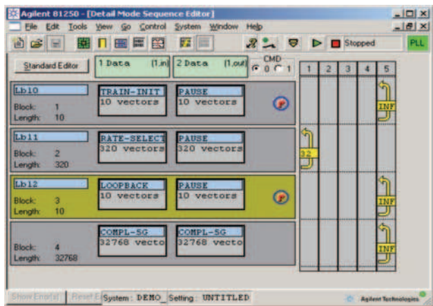
Figure 5. ParBERT detail mode sequence editor screen
