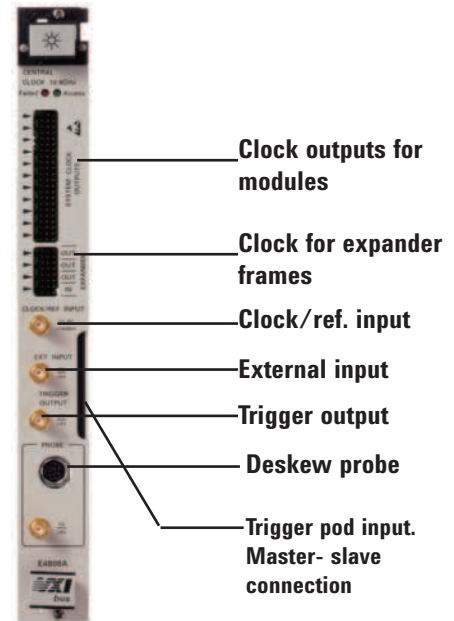
Figure 33: Clock module
