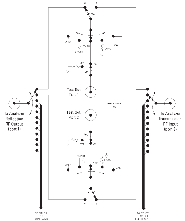
Block diagram for the Agilent 87075C (only one test set port pair is shown)
