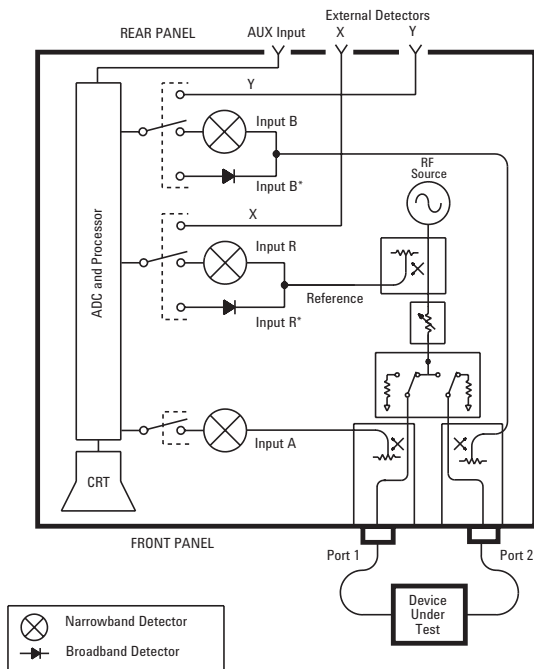
Block diagram for the Agilent 8712ES and 8714ES
