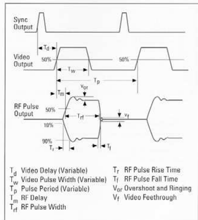
Typical pulse modulation envelope illustrates the fast rise and fall times, excellent flatness and pulse fidelity of the HP 70340A.
