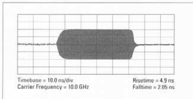
Typical pulse modulation envelope illustrates the fast rise and fall times, excellent flatness and pulse fidelity of the HP 70340A.
