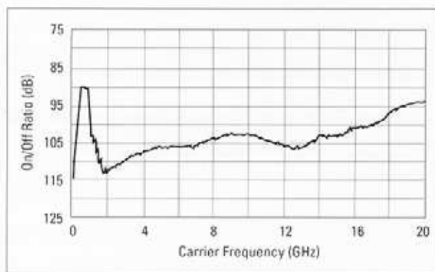
Typical pulse modulation on/off ratio at +8 dBm .
