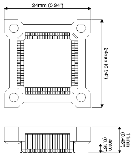
QFP Socket Adapter Dimensions for HP 64784J (HP P/N 64784-61614)
