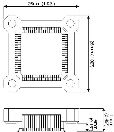
QFP Socket Adapter Dimensions for HP 64784D and G (HP P/N 64784-61612)
