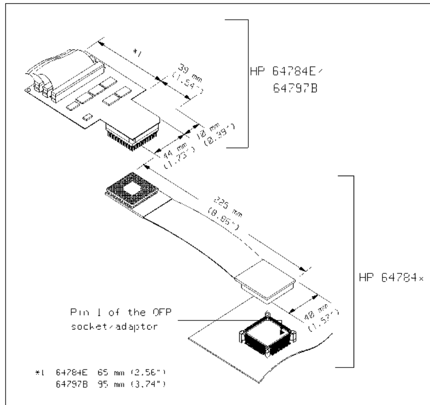
Adapters and Cable Dimensions
