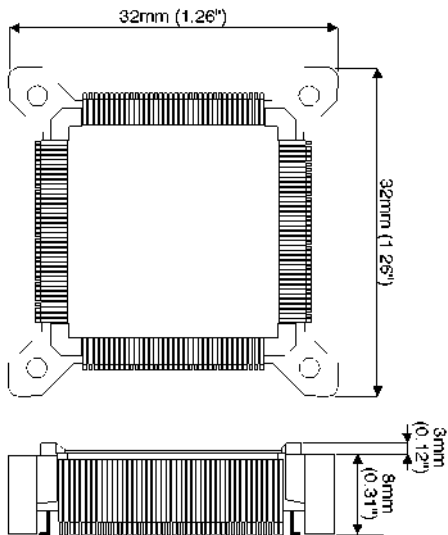
QFP Socket Adapter Dimensions for HP 64784C and F (HP P/N 64784-61611)
