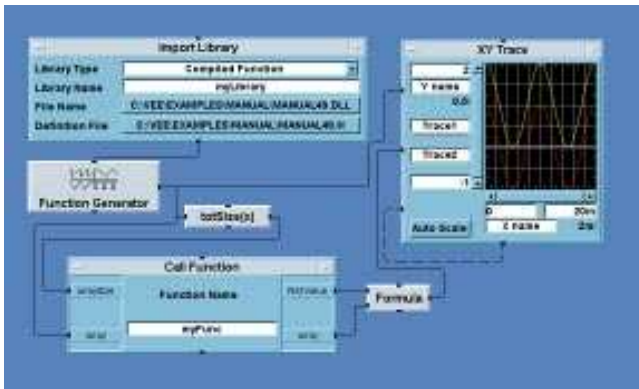
This HP VEE program is calling a C function in a DLL, which adds one to the incoming waveform and returns it to HP VEE.
