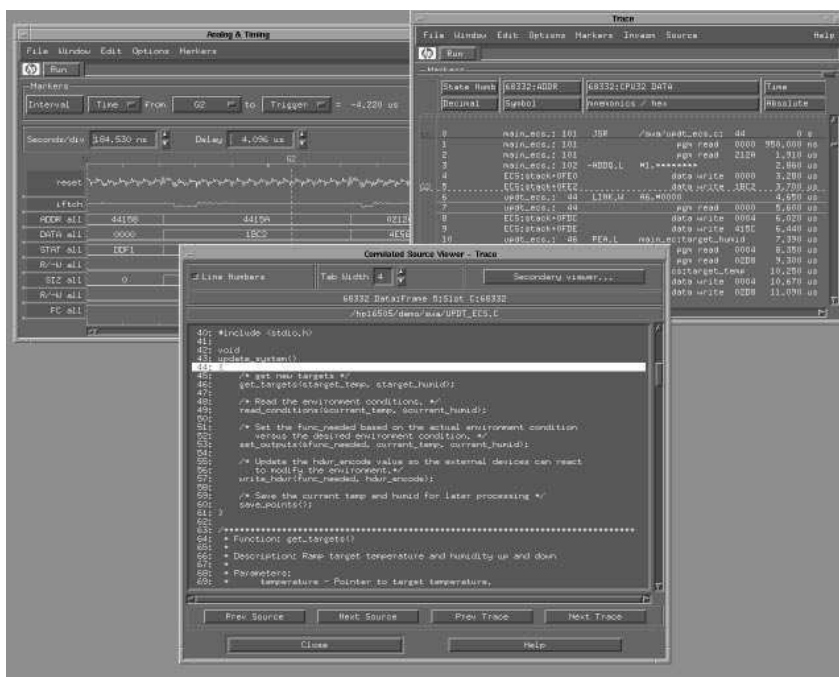
Figure 2. Get a real-time window into system behavior with source code level viewing of executed code.
