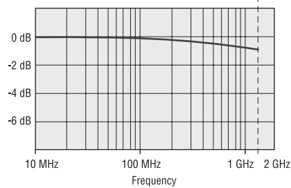
75 Ω Mux Typical AC Performance Graphs
