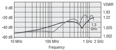
Typical Return Loss/VSWR
