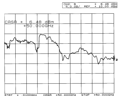
Typical output power available from the Agilent 83599A in normal (versus high power) operating mode
