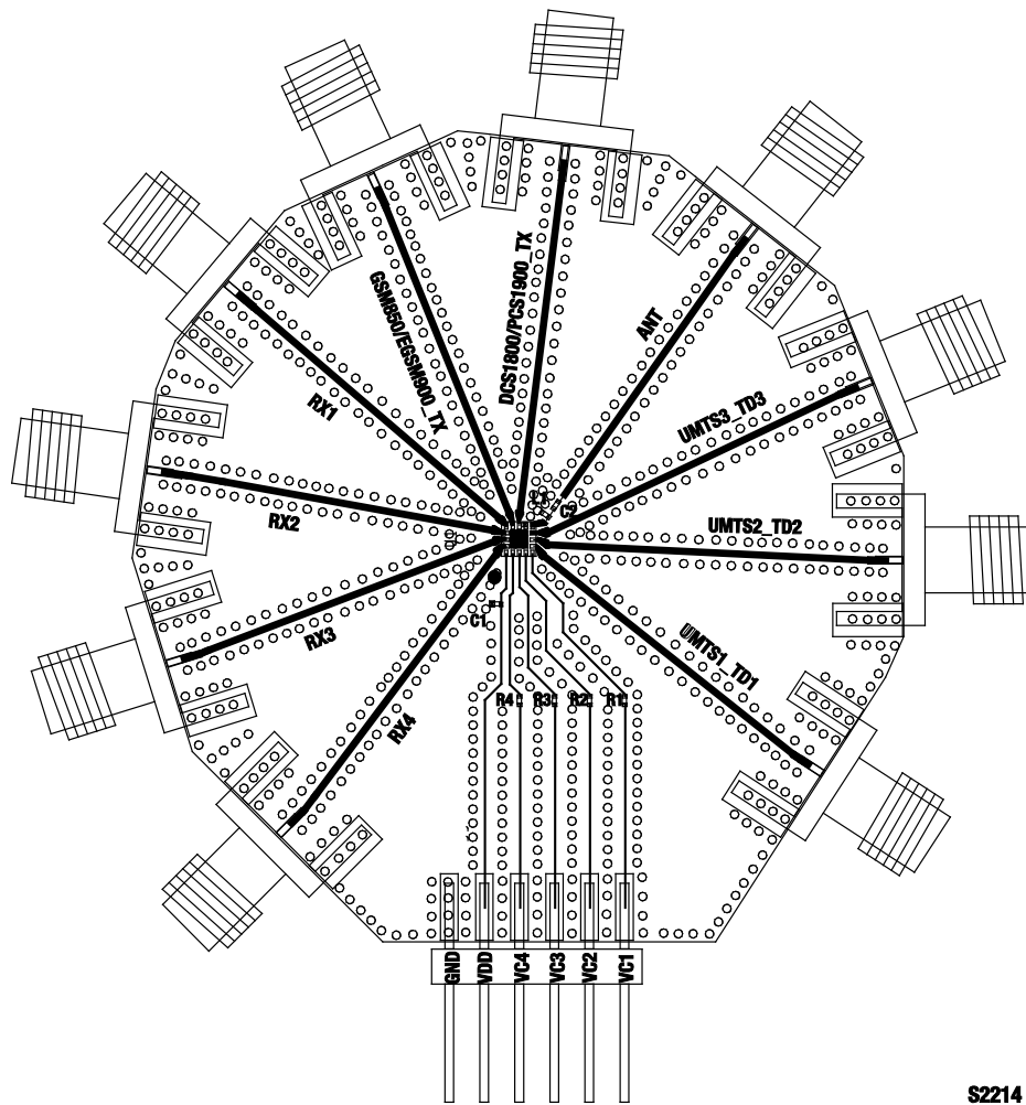
Figure 4. SKY18120-11 Evaluation Board Assembly Diagram
