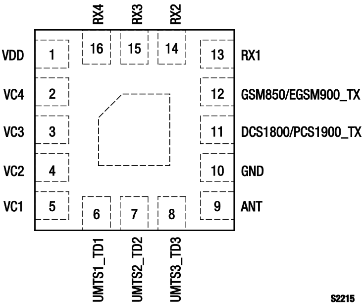
Figure 2. SKY18120-11 Pinout – 16-Pin MCM (Top View)
