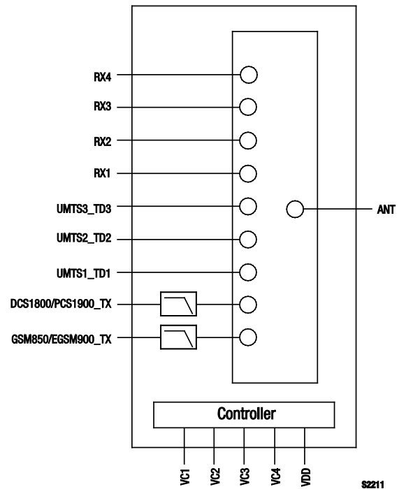
Figure 1. SKY18120-11 Block Diagram
