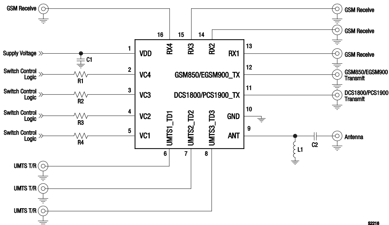
Figure 3. SKY18120-11 Evaluation Board Schematic
